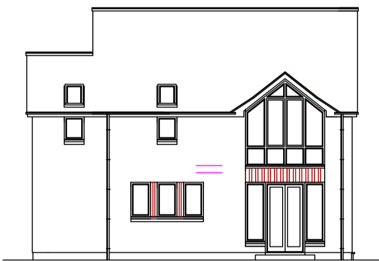
REAR ELEVATION (south west)
